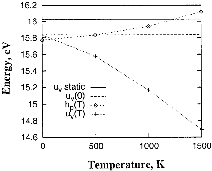
Fig. 3. Temperature variation of h_p ( \diamond ) and u_v (+) for a supercell of MgO containing 216 ions, with one \text{Mg}^{2+} replaced by \text{Ba}^{2+} . u_v(0) and u_v(\text{static}) are also shown.
