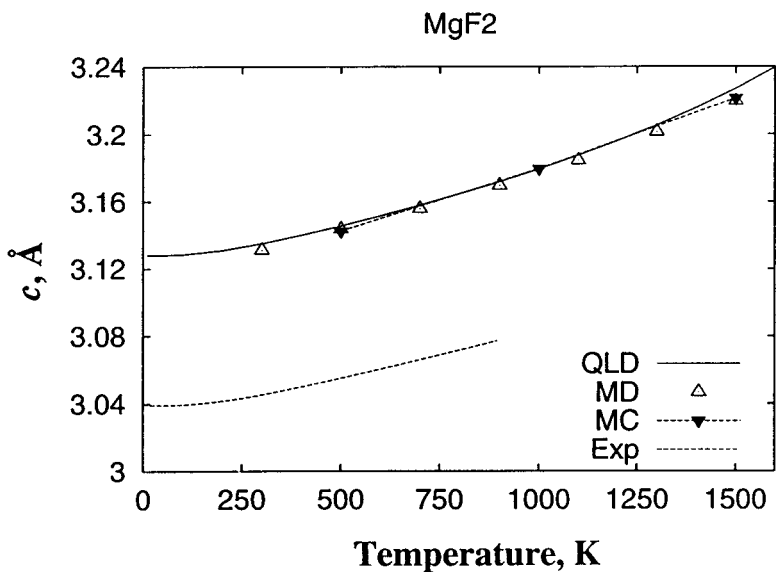
Fig. 1. Calculated values of a and c for MgF 2 , with experimental data from Ref. 11.
