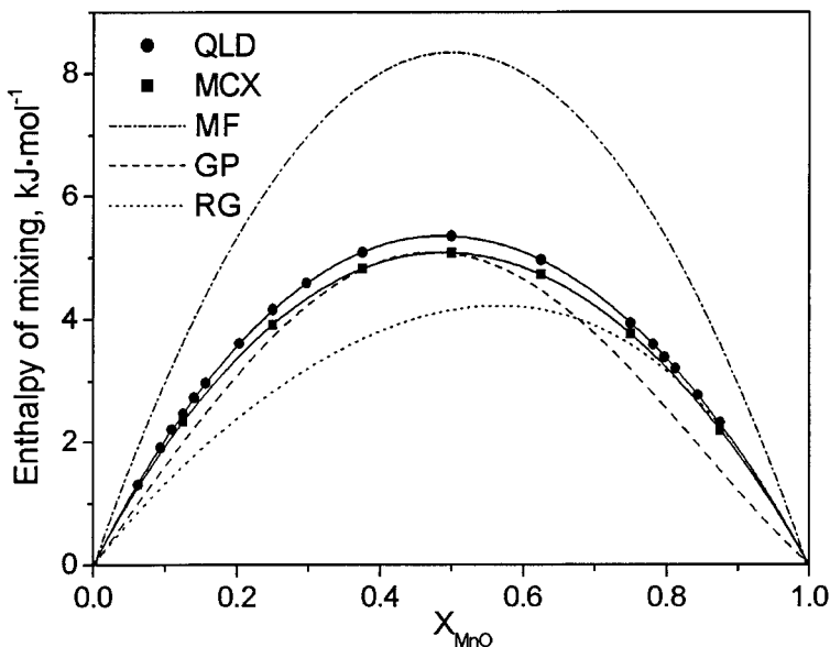
Fig. 4. Calculated values of \Delta H_{\text{mix}} at 1000 K for MnO/MgO given by configurational lattice dynamics (QLD), exchange Monte Carlo (MCX), and mean field theory (MF). Two sets of experimental data are also shown (RG from Ref. 30, GP from Ref. 31).
