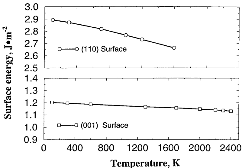
Fig. 2. Calculated surface energies for MgO.
